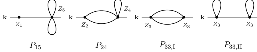
Figure 1: The four topologies of the deterministic two-loop power spectrum, Eqs. (4.1)–(4.5). Each vertex is a kernel, K_n in real space or Z_n^{\text{gal}} in redshift space, of the perturbative order in its subscript; each internal line is one linear power spectrum, and the external lines carry \mathbf{k} . A closed line on one vertex is a momentum pair (\mathbf{q}, -\mathbf{q}) contracted inside one kernel, a tadpole; in P_{24} it is the inner integral I^{(4)} , and P_{33,\text{I}} has none. In P_{15} and P_{33,\text{II}} the line joining the vertices is not integrated over and gives the factor P_{\text{lin}}(k) . Symmetry factors and diagram counts are in Table 2.
