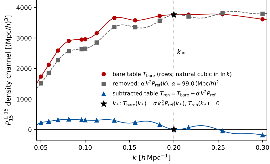
Figure 3: Pivot subtraction, Eq. (6.18), on one two-loop component: the density component of P_{15}^{1,15} ( b_1\gamma_{41} pair, diagram D033, evaluated at f = 0 ) at z = 0.61 . Red circles: bare integral T_{\text{bare}} . Gray squares: removed part \alpha k^2 P_{\text{ref}}(k) , \alpha = 99.0 (\text{Mpc}/h)^2 , with P_{\text{ref}} a fixed reference linear spectrum used in place of P_{\text{lin}} in this illustration. Blue triangles: renormalized component T_{\text{ren}} , an order of magnitude smaller and zero at k_* = 0.2 (dotted line, stars). Curves interpolate in \ln k ; per-point errors (a few times 10^{-3} of T_{\text{bare}} ) are below symbol size. Wavenumbers in h \text{ Mpc}^{-1} , values in (\text{Mpc}/h)^3 .
