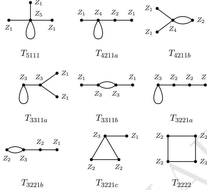
Figure 4: The nine one-loop contraction types of the redshift-space galaxy trispectrum, drawn as connected multigraphs on the four kernel vertices Z_n = Z_n^{\text{gal}} with four internal lines, each standing for a linear power spectrum; every vertex also carries one external momentum, not drawn. The one independent cycle of Eq. (10.7) is a self-loop ( \mathbf{q}, -\mathbf{q} ) inside one kernel ( T_{5111} , T_{4211a} , T_{3311a} , T_{3221a} ), a doubled line ( T_{4211b} , T_{3311b} , T_{3221b} ), a triangle ( T_{3221c} ) or a square ( T_{2222} ). Subscripts give the kernel-order partition of Eq. (10.2), letters distinguish the types within a partition, and the integrands are those of Eq. (10.9).
