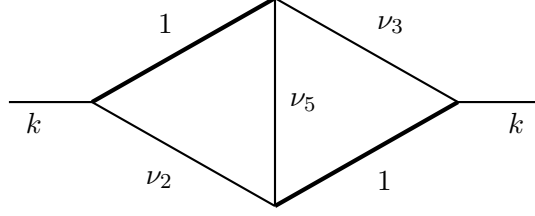
Figure 2: The two-loop kite master integral, Eq. (5.2) at d = 3 , for the non-adjacent family K(1, \nu_2, \nu_3, 1, \nu_5) : the external momentum k enters and leaves at the side vertices, the internal lines carry \nu_1, \dots, \nu_5 in the routing of the text ( \nu_4 upper left, \nu_1 lower right), and the two unit indices sit on the thick lines, which share no vertex. Patterns with the unit indices on adjacent lines have closed forms in Gamma functions and single hypergeometric sums [52]; this non-adjacent family is the one pattern without such a form [39], and Eq. (5.4), derived in the Supplementary Information, Sec. S3, gives it in closed form with two additional single sums.
